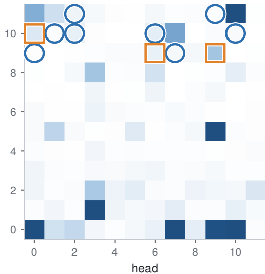
intact-state single ablation
