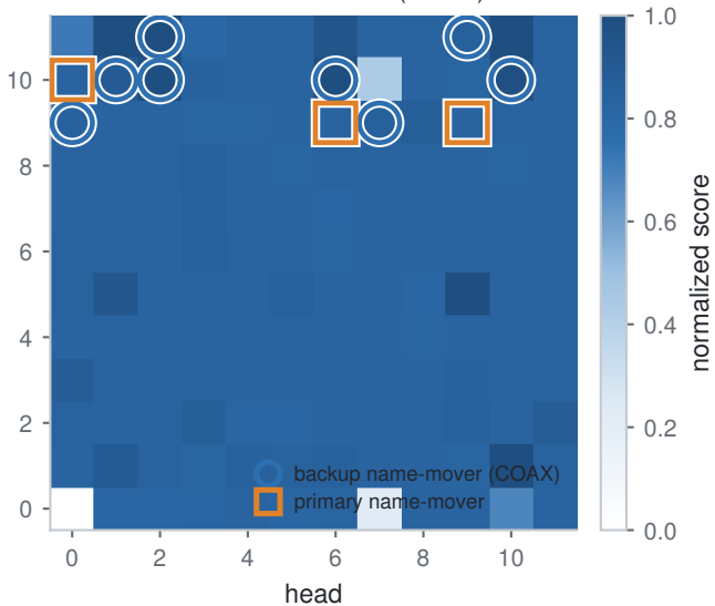
conditional co-ablation (COAX)
